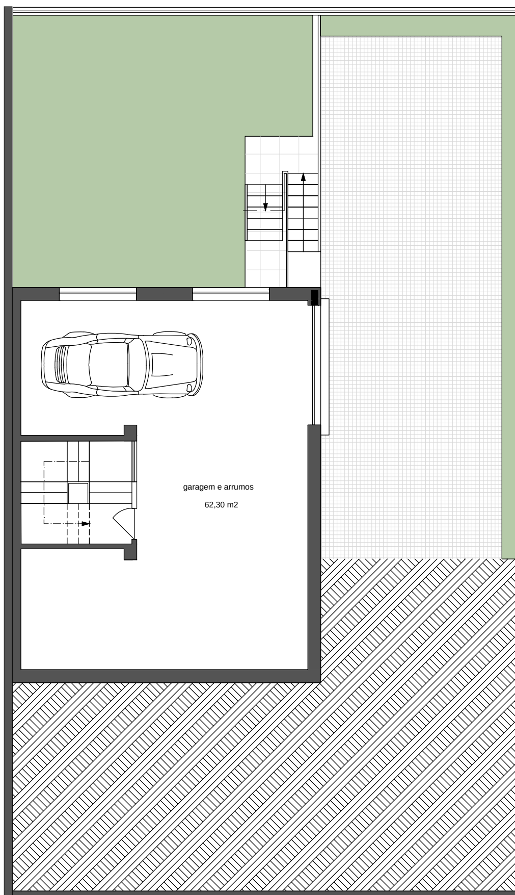
Planta do Lote02 CAVE
